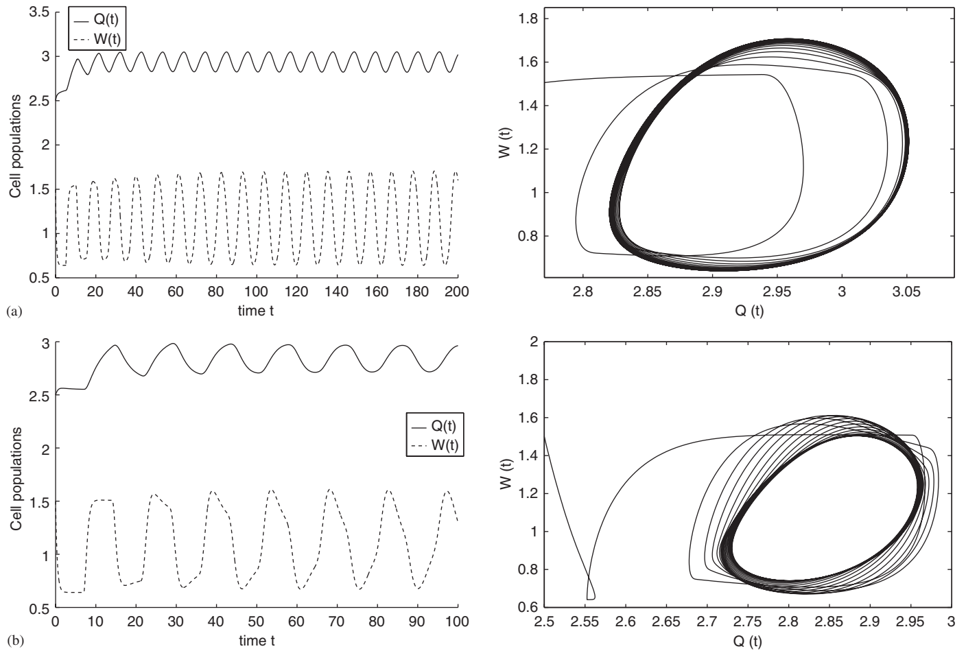
Fig. 4. Oscillating solutions with \tau_1 close to zero. Parameters are given by (18) and (19), with A = 20 . The time delays are \tau_1 = 0.05 and (a) \tau_2 = 5 days and (b) \tau_2 = 7 days. Oscillating solutions appear with periods about (a) 10 days for the white blood cell population (the dashed line) as well as for the hematopoietic stem cell population (solid line), and (b) 15 days for the two cell populations, with very low values attained by the white blood cell count, as observed in cyclical neutropenia. The steady state (Q^*, W^*) of (2) is unstable in both cases. Note that the time scales are different from one picture to another.
