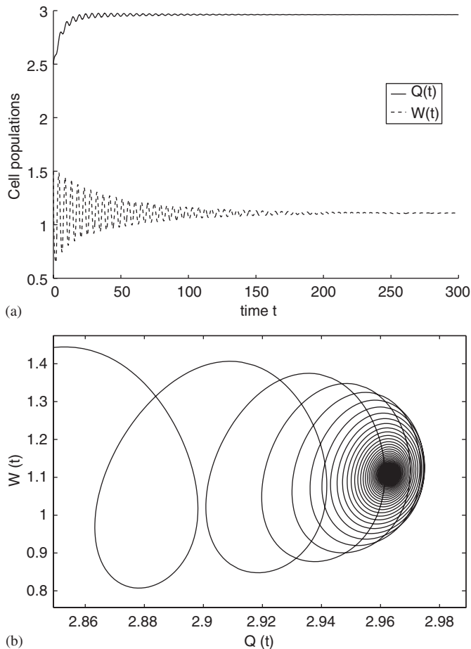
Fig. 3. Asymptotic stability. The steady state (Q^*, W^*) of (2) is locally asymptotically stable, even though damped oscillations can be observed. In figure (a), the solid line is for the hematopoietic stem cell population Q(t) and the dashed one is for the white blood cell population W(t) . In figure (b), the solutions are drawn in the (Q, W) -plane. Parameters are given by (18) and (19), with A = 20 . The time delays are \tau_1 = 0.05 and \tau_2 = 2 days.
