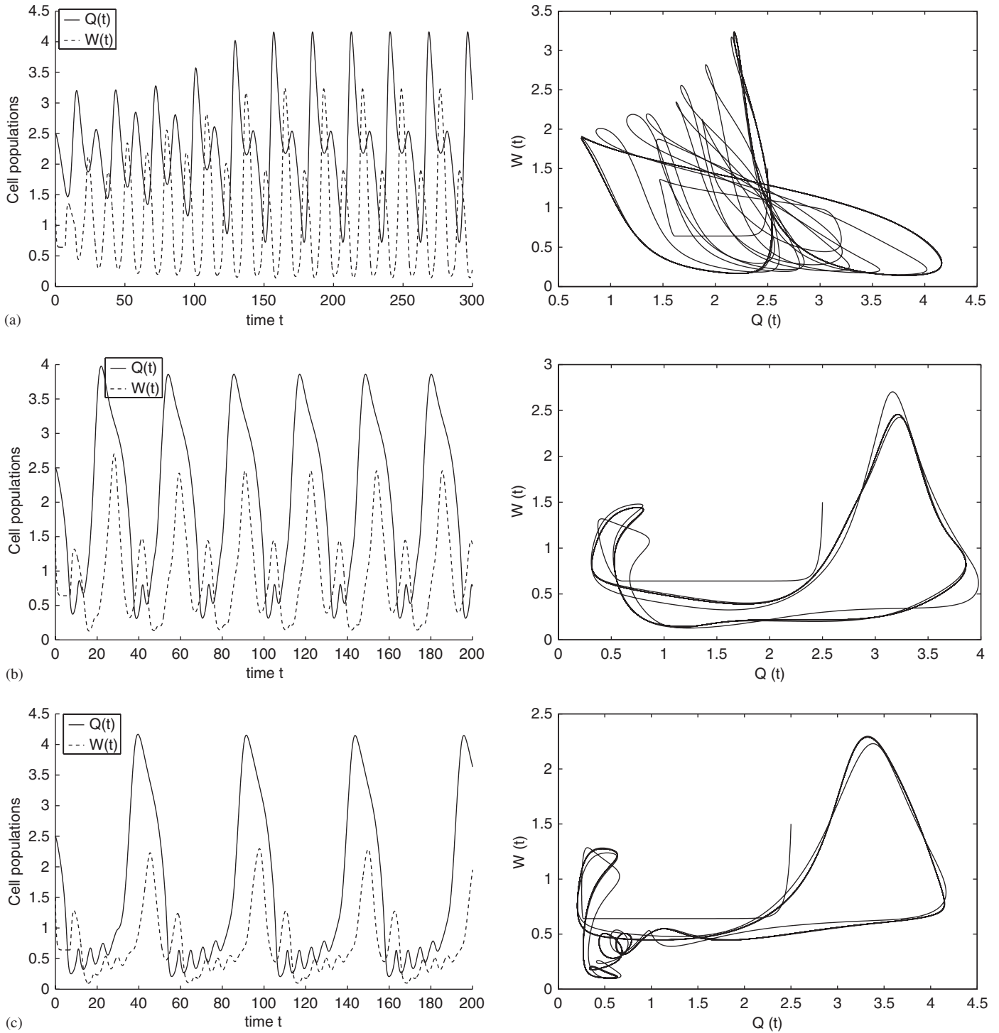
Fig. 5. Long period oscillations. The solid line represents the hematopoietic stem cells population and the dashed line the white blood cell population. Parameters are given by (18) and (19), with A = 20 . The time delays are (a) \tau_1 = 3 days, (b) \tau_1 = 4 days, (c) \tau_1 = 5 days, with \tau_2 = 7 days in the three cases. Oscillating solutions with periods in the range of (a) 20–25 days, (b) 30 days and (c) 50 days, for the two cell populations, are observed, that can be related to oscillations observed in cyclical neutropenia (see Bernard et al., 2003). Ripples can be observed in the two populations in figure (c).
