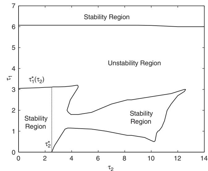
Fig. 2. Stability diagram. Stability of the steady state (Q^*, W^*) of system (2) is displayed as a function of \tau_1 and \tau_2 . The full lines are the boundaries between stable and unstable regions. This diagram was obtained using the values mentioned in Section 4, in (18) and (19), with A = 20 . In this case, the steady state (Q^*, W^*) of system (2) no longer exists when \tau_1 \geq 7 days, and the critical value \tau_2^* obtained in Theorem 5 equals 2.5 days and is indicated on the figure. The more biologically relevant area for \tau_1 and \tau_2 corresponds to small values of the two parameters, close to one day. It is a stable region given by Theorem 7 (bounded by the vertical dotted line \tau_2 = \tau_2^* and the curve \tau_1 = \tau_1^*(\tau_2) ). However, one can note very rich dynamics of the steady state. As \tau_1 (respectively, \tau_2 ) increases, a finite number of stability switches may occur.
