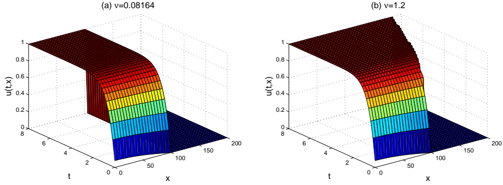
Figure 3: A comparison of densities of winged female mosquitoes between (a) small advection and (b) large advection. Here \mu = 0.5 , and other parameters are given in (6.1).
