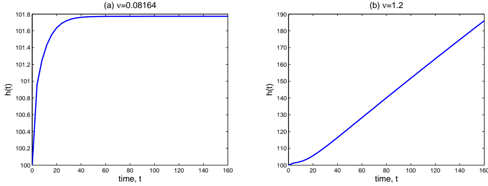
Figure 4: A comparison of free boundary movement between (a) small advection and (b) large advection. Here \mu = 0.5 , and other parameters are given in (6.1).
