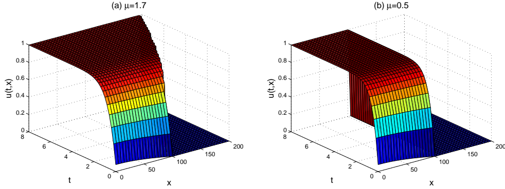
Figure 1: A comparison densities of winged female mosquitoes between (a) large invasive ability and (b) small invasive ability. Here \nu = 8.164 \times 10^{-2} , and other parameters are given in (6.1).
