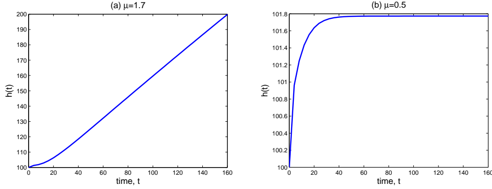
Figure 2: A comparison of free boundary movement between (a) large invasive ability and (b) small invasive ability. Here \nu = 8.164 \times 10^{-2} , and other parameters are given in (6.1).
