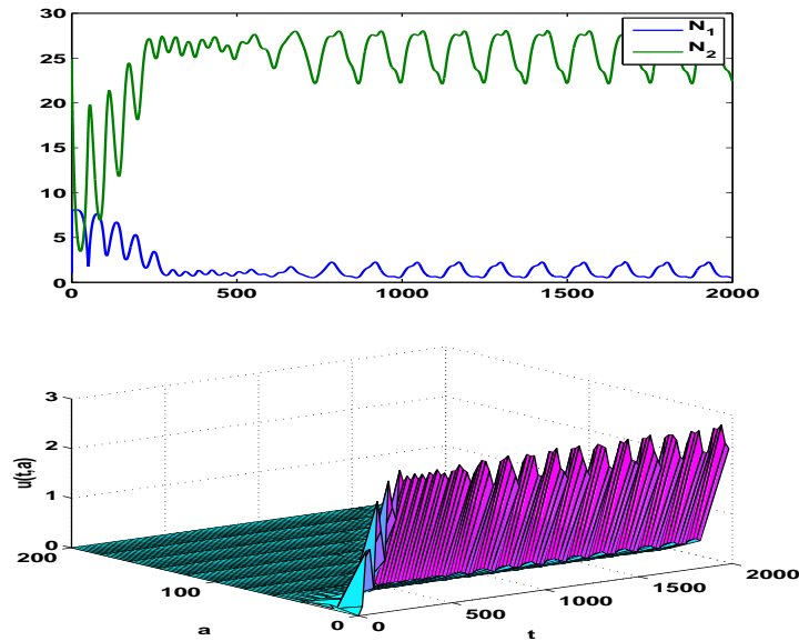
FIGURE 2. Numerical simulations of system (1) with \tau = 50 . (a) Time series of N_1(t) (lower blue curve) and \int_0^{+\infty} N_2(t, a) da (upper green curve) which are oscillatory about their equilibrium values. (b) The age distribution of N_2(t, a) which is periodic in time.
