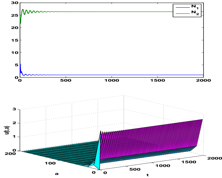
FIGURE 1. Numerical simulations of system (1) with \tau = 10 . (a) Time series of N_1(t) (lower blue curve) and \int_0^{+\infty} N_2(t, a) da (upper green curve) which converge to their equilibrium values. (b) The age distribution and time series of N_2(t, a) .
