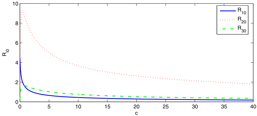
Fig. 1 The curves of the basic reproduction number of patch i , \mathcal{R}_{i0} , versus c
