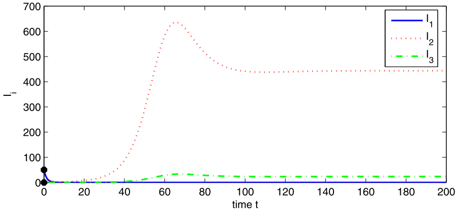
Fig. 2 Numerical simulations of system (2a) showing I_i vs. t . Initial conditions: S_1(0) = 1800 , I_1(0) = 50 , R_1(0) = 100 , V_1(0) = 0 , and S_2(0) = I_2(0) = R_2(0) = V_2(0) = S_3(0) = I_3(0) = R_3(0) = V_3(0) = 0 . \mathcal{R}_{10} < 1 , \mathcal{R}_{20} > 1 , and \mathcal{R}_{30} > 1
