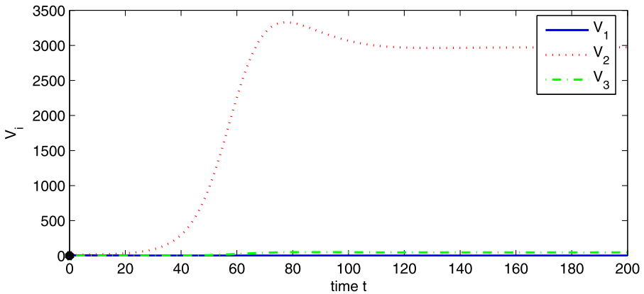
Fig. 3 Numerical simulations of system (2a) showing V_i vs. t . Initial conditions: S_1(0) = 1800 , I_1(0) = 50 , R_1(0) = 100 , V_1(0) = 0 , and S_2(0) = I_2(0) = R_2(0) = V_2(0) = S_3(0) = I_3(0) = R_3(0) = V_3(0) = 0 . \mathcal{R}_{10} < 1 , \mathcal{R}_{20} > 1 , and \mathcal{R}_{30} > 1
